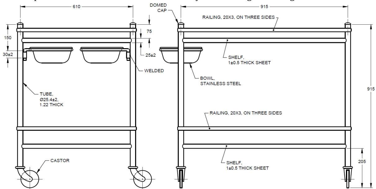
Fig. 1 MEDICINE TROLLEY
